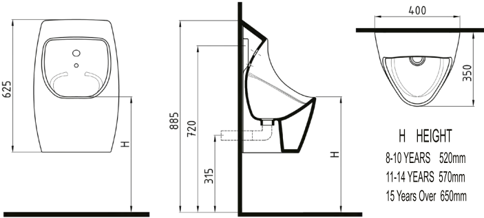
URINAL 62 cm REAR INLET WITH PHOTOCELL-BATTERY HRPS06201VSAW5000 URINAL 62 cm REAR INLET WITH PHOTOCELL-ELECTRIC HRPS06202VSAW5000
