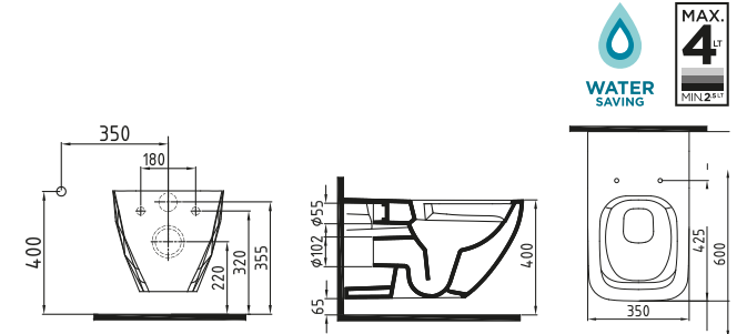
WALL HUNG WC PAN 60 cm NO-RIM/ CONCEALED FIXING KRKA060N1VP0W3000 600x350mm
