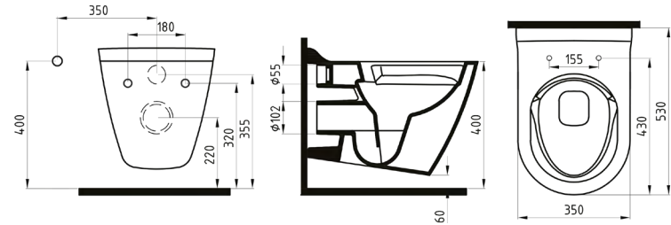
MINERAL W.HUNG WC PAN 52 cm NO-RIM WHITE MNKA052N1VP0W3000 530x350mm
