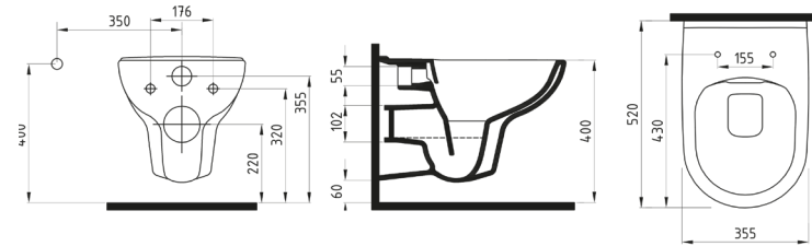
WALL HUNG WC PAN 52 cm LEKA052H2VPOW5000 520x355mm
