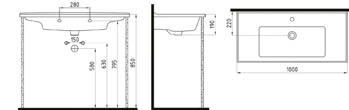
VANITY WASHBASIN 100 cm SINGLE HOLE NPLK10001FD1W5000 1000x470mm
