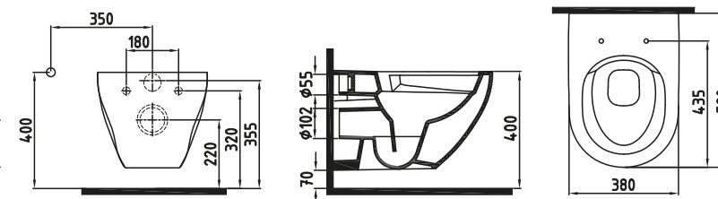
WALL HUNG WC PAN 52 cm NO-RIM/ CONCEALED FIXING DNKA052N1VP0W3000 520x380mm
