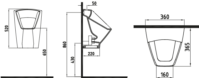
URINAL 52 cm REAR INLET NPPS05201VSAW3000 520x365mm
