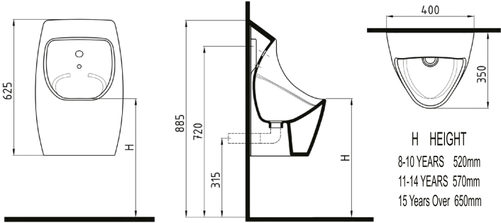
URINAL 62 cm REAR INLET WITH PHOTOCELL-BATTERY HRPS06201VSAW5000
