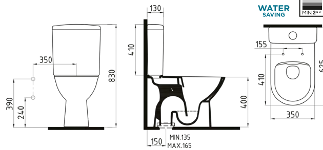
CISTERN 41 cm BOTTOM INLET CPRS04101VDAW5000 410mm
