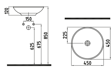
COUNTERTOP WASHBASIN 45 cm WITHOUT HOLE HRLG04501FDOW5000 Ø450mm
