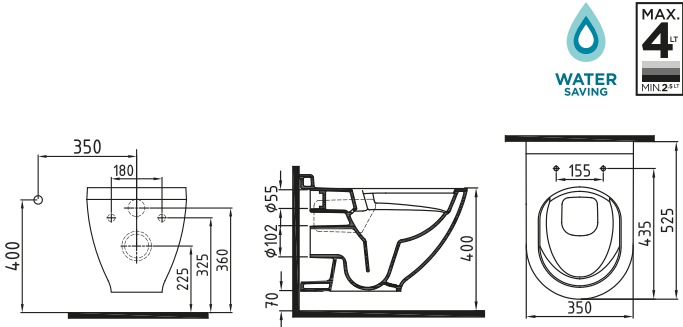
WALL HUNG WC PAN 52 cm NO-RIM HRKA052N2VPOW3000 520x350mm
