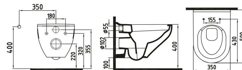
WALL-HUNG WC PAN 50 cm NO-RIM IOKA050N2VPOW5000 500x350mm
