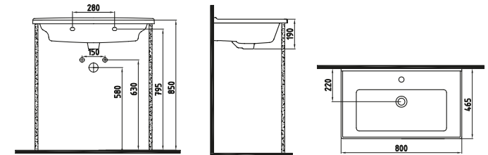
VANITY WASHBASIN 80 cm SINGLE HOLE NPLK08001FD1W5000 800x470mm
