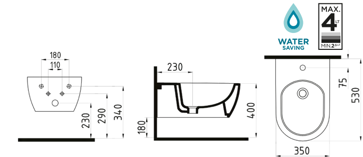
WALL HUNG BIDET 52 cm N3 SINGLE HOLE HRBA05203VD1W3000 530x350mm
