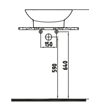
COUNTERTOP WASHBASIN 46 cm SINGLE HOLE HRLG04601FD1W5000 460x550mm
