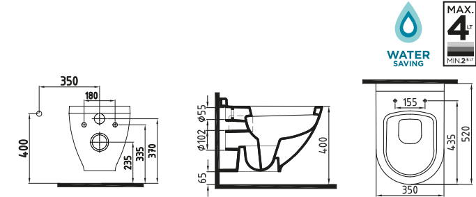
WALL HUNG WC PAN 52 cm HRKA052AMVPOW5000 520x350mm
