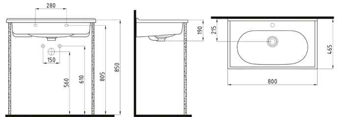
VANITY WASHBASIN 80 cm SINGLE HOLE FELK080B1FD1W5000 800x465mm
