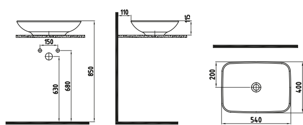
COUNTERTOP WASHBASIN 54 cm WITHOUT HOLE HRLG05401FDOW5000 540x400mm
