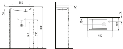
INFINITIUM VANITY WB. 45 CM SINGLE HOLE INLK04501FD1W5000 450mm
