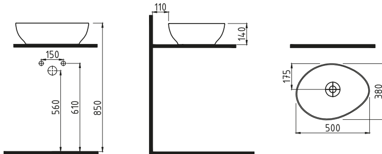
ASYMMETRIC COUNTERTOP WASHBASIN 50 cm WITHOUT HOLE MTLG05004FDOW5000 500x380mm
