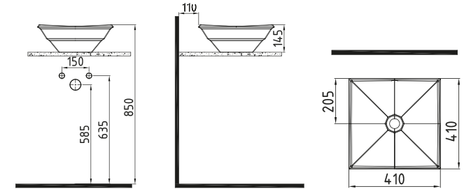
COUNTERTOP WASHBASIN 41 cm WITHOUT HOLE KRLG04101FDOW5000 410x410mm
