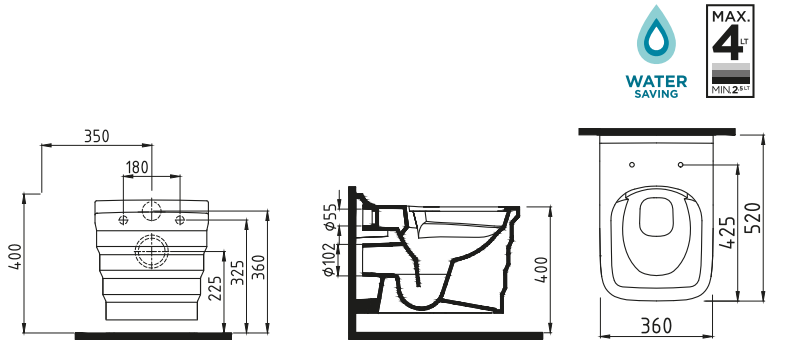
WALL HUNG WC PAN 52 cm NO-RIM/ CONCEALED FIXING SHKA052N1VPOW3000 520x360mm
