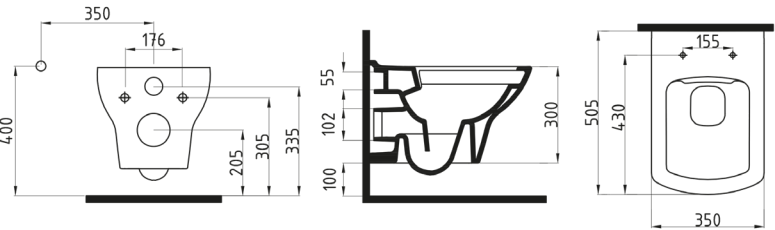
WALL-HUNG WC PAN 50 cm NO-RIM DRKA050N2VP0W5000 500x350mm
