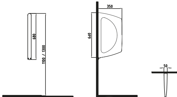
WALL SEPERATOR 68 cm NPPA06801V00W3000 680x350mm
