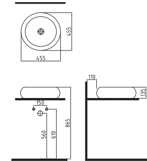
COUNTERTOP WASHBASIN 46 cm WITHOUT HOLE DIAMONT BLUE COATED FALG04601FD0D0SZ0 Ø 460mm
