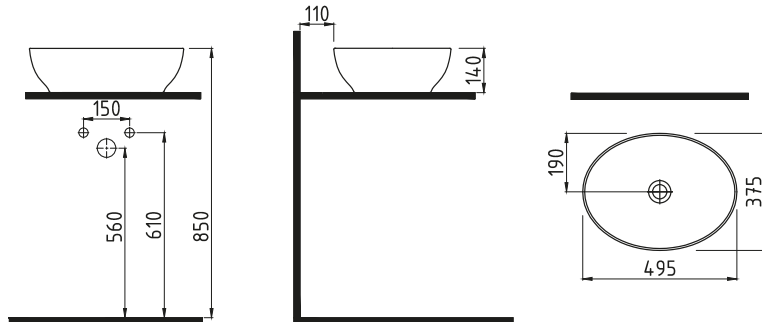
OVAL COUNTERTOP WASHBASIN 50 cm WITHOUT HOLE MTLG05002FDOW5000 495x375mm
