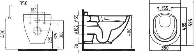
WALL HUNG WC PAN 52 CM NO-RIM CONCEALED FIXING HRKA052N5VP0W3000 520x350mm
