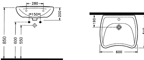
SINGLE PIECE DISABLED WASHBASIN 60 cm SINGLE HOLE TPLE06001VD1W3000 600x510mm
