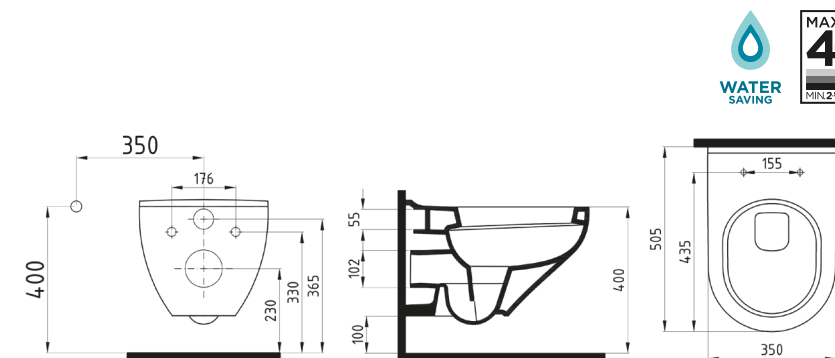
WALL-HUNG WC PAN 50 cm IOKA050AMVPOW5000 500x350mm
