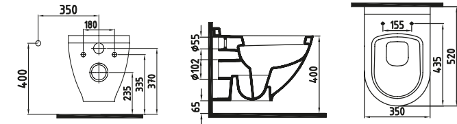
WALL HUNG WC PAN 52 cm NO-RIM CONCEALED FIXING HRKA052GMVP0W3000 520x350mm
