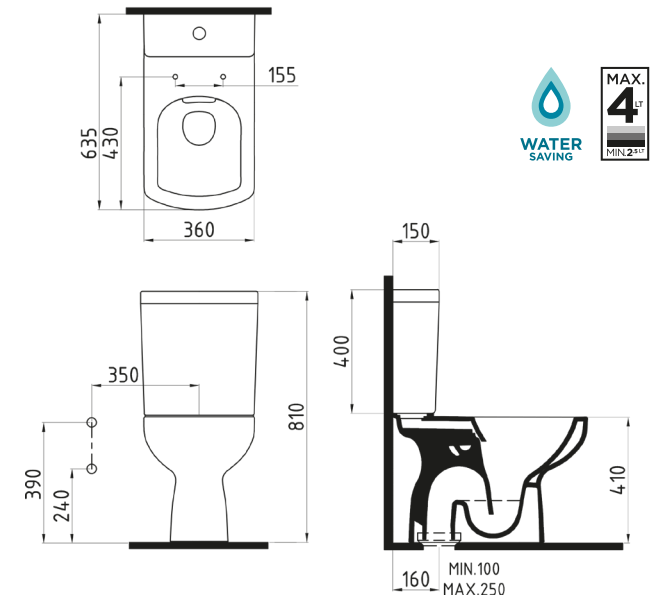
CISTERN 39 cm BOTTOM INLET DRRS039B1VDAW5000 390mm
