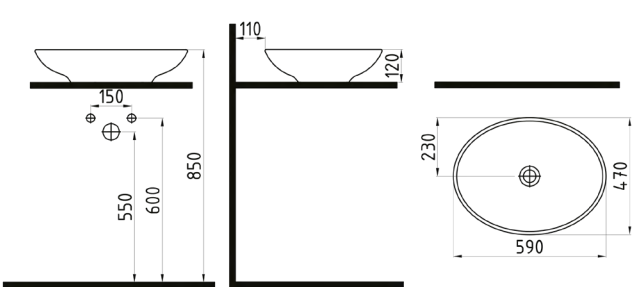
COUNTERTOP WASHBASIN 59 cm WITHOUT HOLE HRLG05901FDOW5000 590x470mm
