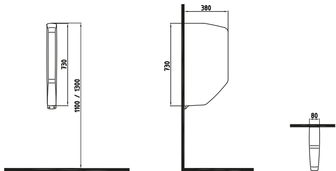
WALL SEPERATOR 73 cm NPPA07301V00W3000 730x380mm
