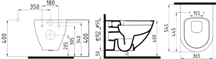
WALL HUNG WC PAN 54 CM NO-RIM CONCEALED FIXING HRKA054H1VP0W5000 540x365mm *Suitable WITH AMARO Seat Cover
